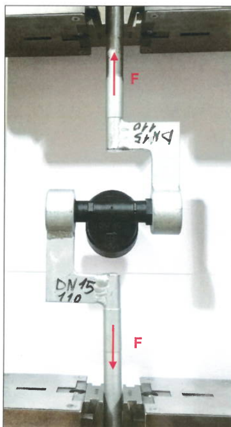
Photo 1 - Test configuration
